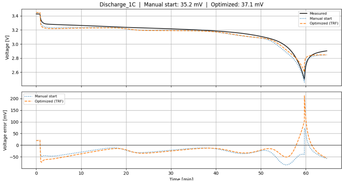
Figure 8 – Discharge 1C. Slightly worse (35.2 → 37.1 mV) with a +210 mV spike at the knee: the discharge is only 1 of 9 terms, so the optimizer favours the charge tests.
