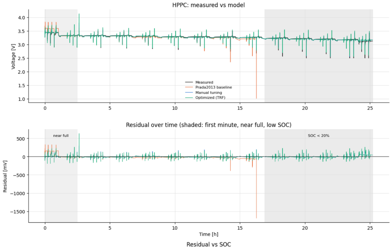
Figure 9 – HPPC, three parameter sets. Both tuned sets cover the full profile; the optimized set's largest error is a 630 mV spike during a 20 A charge pulse at about 96 % SOC.
