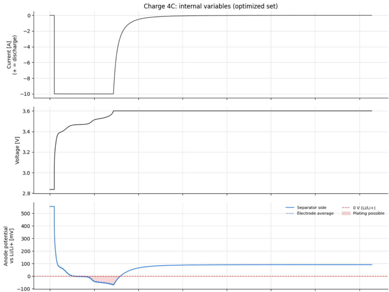
Figure 13 - Charge 4C. The anode stays below 0 V for about 10 minutes, then recovers to about 90 mV once the current tapers.
