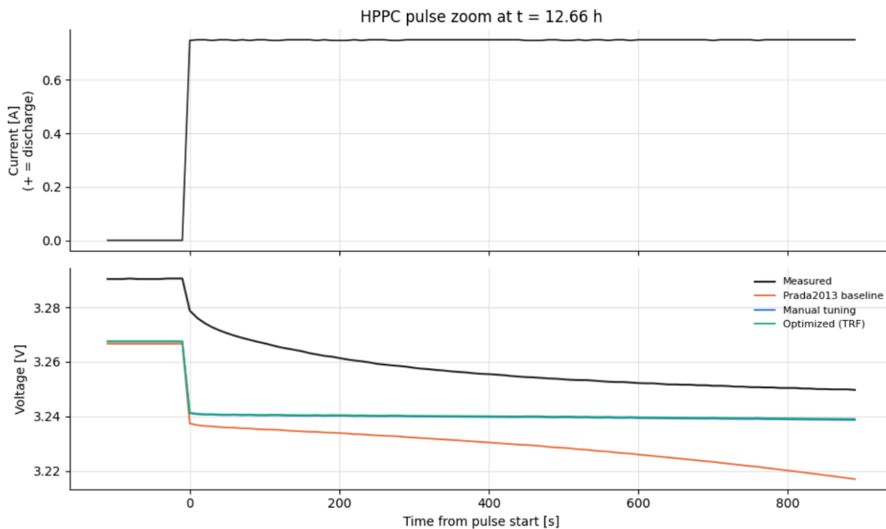
Figure 11 – 0.75 A step at 12.66 h. All models sit about 22 mV below the measured rest voltage, and they miss the slow 30 mV sag after the step.
