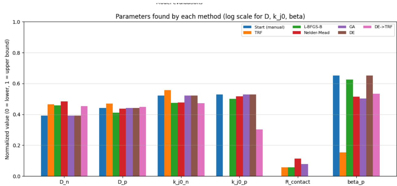
Figure 6 - Parameters, normalized between bounds. D n rises consistently to about 2.5 \cdot 10^{-14} m 2 /s; k j0_p , β p and R contact spread widely at similar J, so only their combined effect is identifiable.
