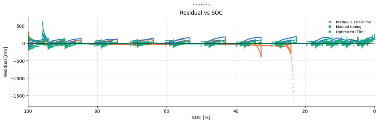
Figure 10 – Residual vs SOC. The optimized set reduces the pulse arcs at mid and low SOC but has its largest errors above 90 % SOC, where k_{j0\_p} = 0.1 and an almost empty LFP surface ( y = 0.001 ) inflate the overpotential.
