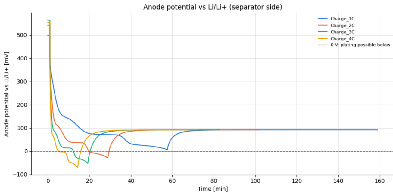
Figure 12 – Anode potential vs \text{Li/Li}^+ . It drops below 0 V (plating possible) from 2C upward, at the end of the CC phase; at 1C the margin is only 6.5 mV.
