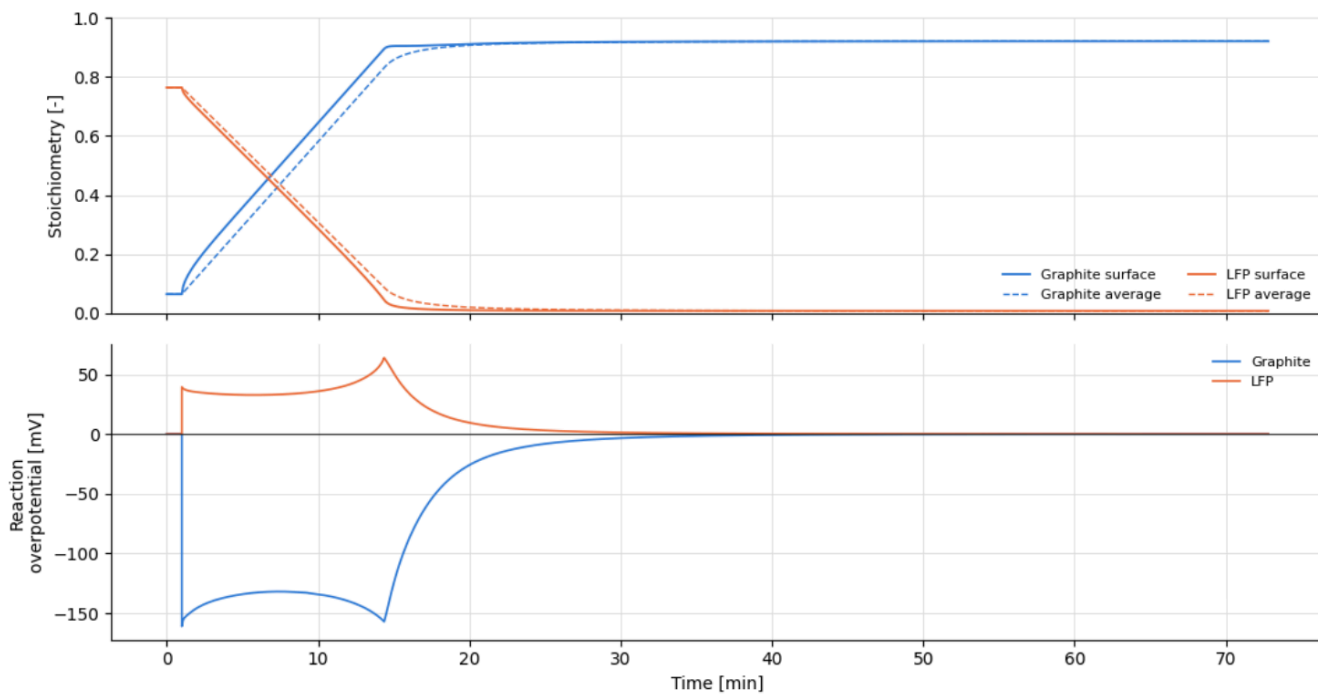
Figure 14 – Charge 4C stoichiometries and overpotentials. The graphite overpotential (130–160 mV) is the largest loss; the LFP surface empties before its average, which starts the CV phase.
